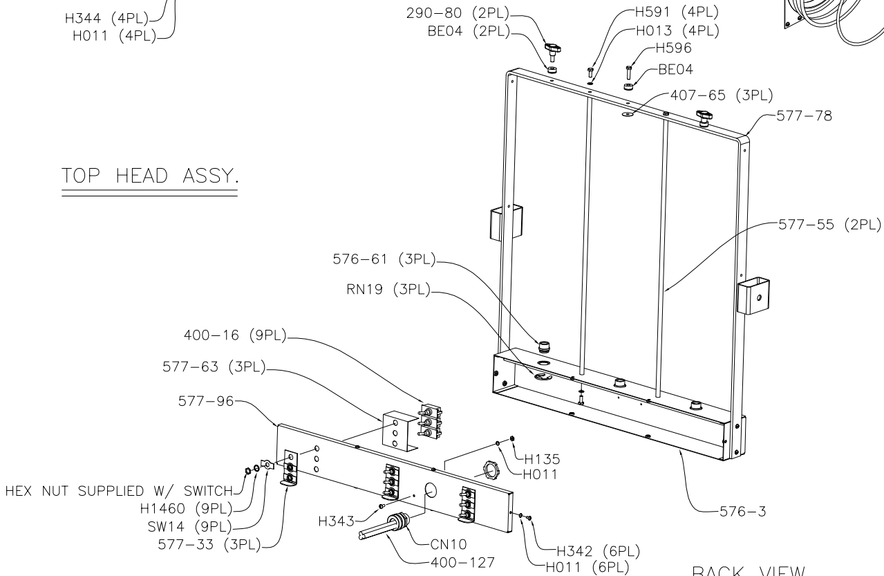
BACK VIEW
