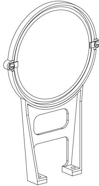
MIRROR ASSY.
