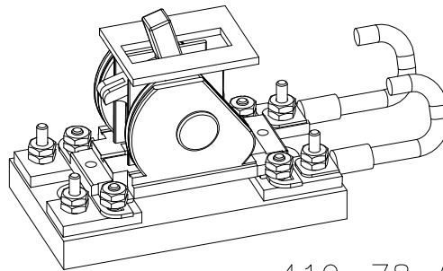
419-78 ASSY.
